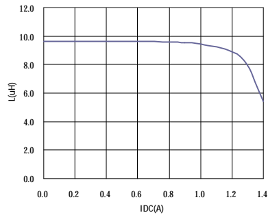
SR0302101KL□
