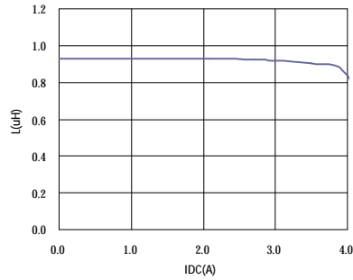
SR0302100ML□
