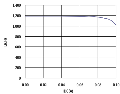
SR0302122KL□
